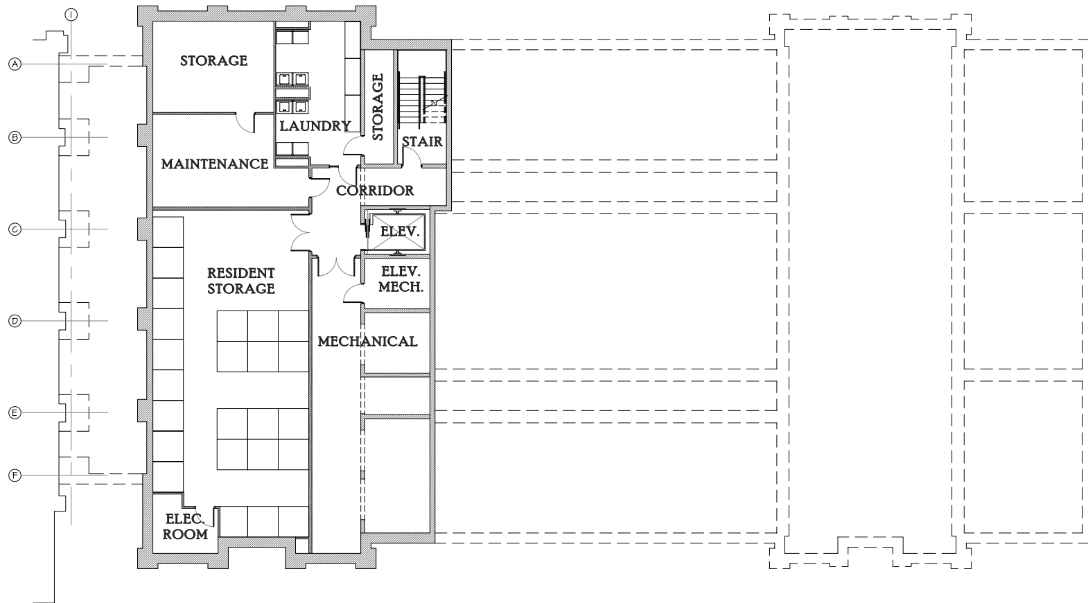
BASEMENT PLAN
